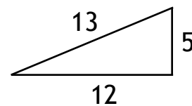
A Classic Right Triangle
